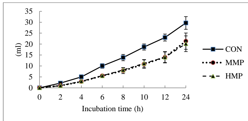
Figure 1 Effect of MP on the volume (mL) of in vitro gas production CON: 50% concentrate + 50% alfalfa without MP; MMP: 50% concentrate + 25% alfalfa + 25% MP; HMP: 50% concentrate + 50% MP.
