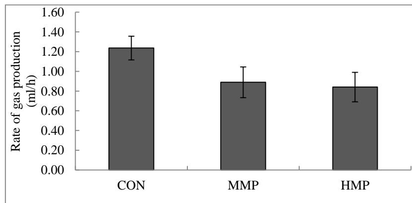
Figure 2 Effect of MP on the rate (mL/h) of in vitro gas production CON: 50% concentrate + 50% alfalfa without MP; MMP: 50% concentrate + 25% alfalfa + 25% MP; HMP: 50% concentrate + 50% MP. Different letters denote significant differences at P < 0.05 . Error bar = 1 SE
